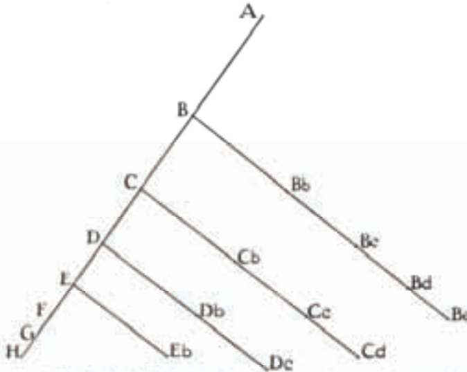
Fig. 7. Evolution by differentiation. Each genus is supposed to survive the whole way along the line at right angles to its origin, e.g. A still survives at H , B at Bc , and so on. In order to save complication, the lines to show the growth Bb , Bc , &c. are not shown.
